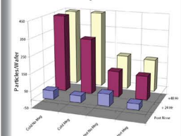
Sulfuric Residue Tests for Various Rinse Processes (Figure 2)
